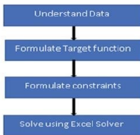
Fig. 1 Methodologyflowchar
