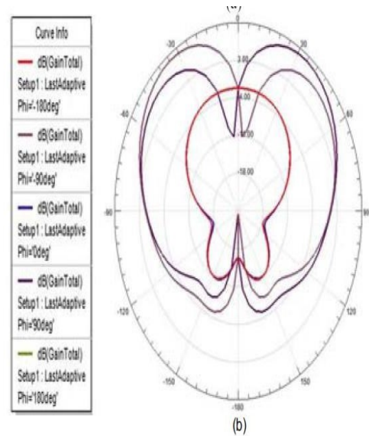
Fig.4 Simulated Radiation pattern of the proposed antenna at (a) 2.5GHz and (b) 5.27GHz
