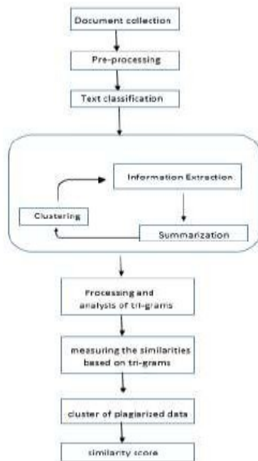
Fig. 3. Proposed Methodology
