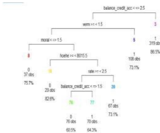
Fig. 4. Decision Tree
