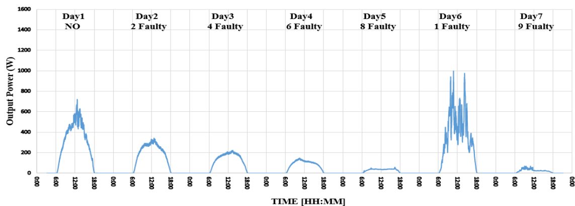
Figure 13. Total output power of PV system for week two under overcast conditions.
