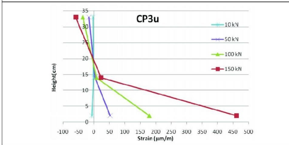
Figure 6: Position of Neutral Axial Versus Applied Load for CP3u
