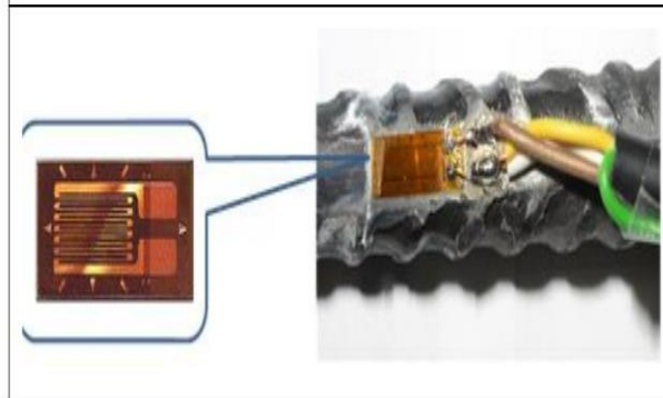
Figure 3: Detail of bonded and welding of electric gauge
