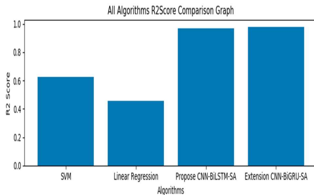
Fig2 comparative analysis of the R 2 score
