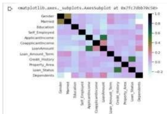
Fig.11. Correlation matrix
