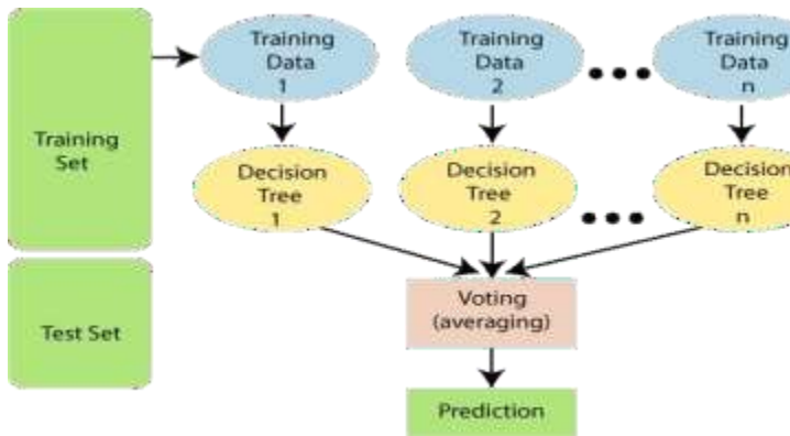
Fig No.3 Random Forest Flow Chart
