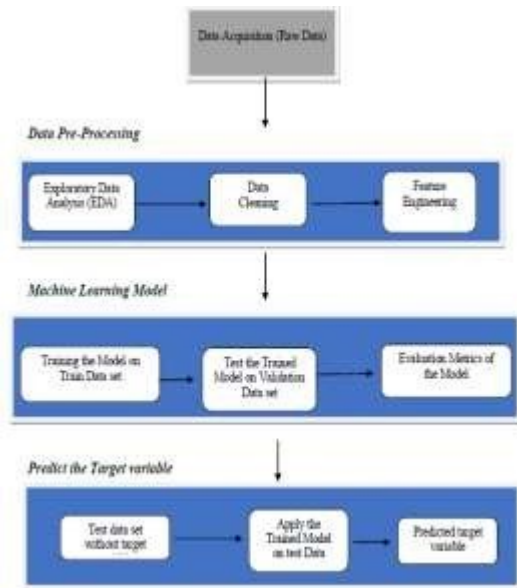
Figure 2. Framework for Machine learning Model
