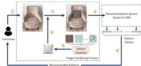
Fig. 1. The proposed recommendation system architecture.
