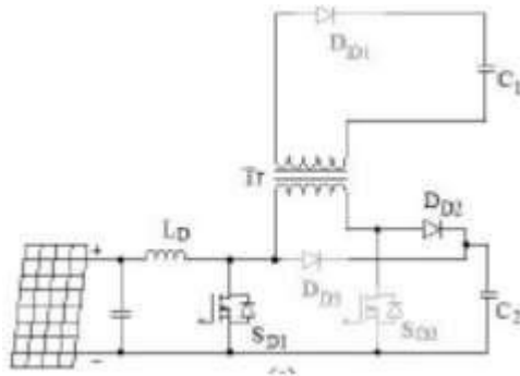
Fig.2 Operation of DC-DC power converter with SD1 switch on condition.
