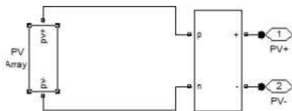
Fig.6 PV Array with DC-to-DC converter.
