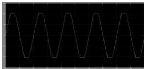
Fig.9 Phase A 7 level output voltage.
