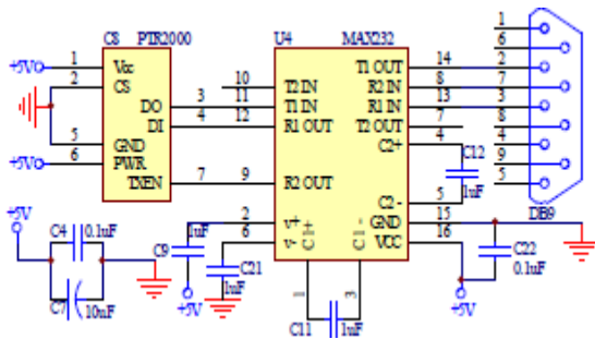
Fig.6 shows a PTR2000 module linked to a MAX232 MSP430F135 sending transaction data to a host computer and receiving commodities data from a weight scale via an RS232 connection.
