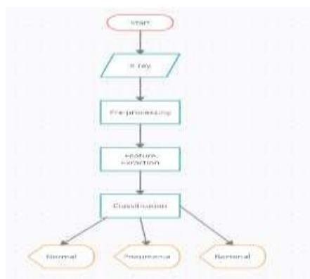
Fig 3.1 Architectural flow
