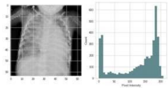
Fig 5.1 Pixel Intensity
