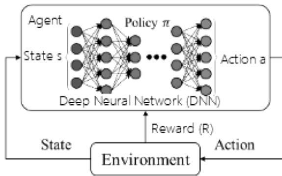
Fig. 5 Schematic structure of deep reinforcement learning (DRL) highlighting a deep neural network
