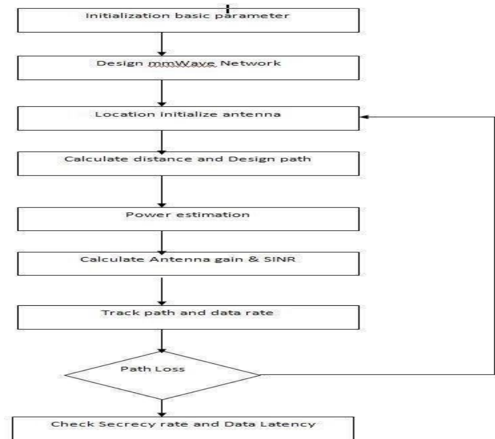
The detailed architecture of the entire suggested working is depicted in Figure 2. First, configure all of the core mmwave settings.
