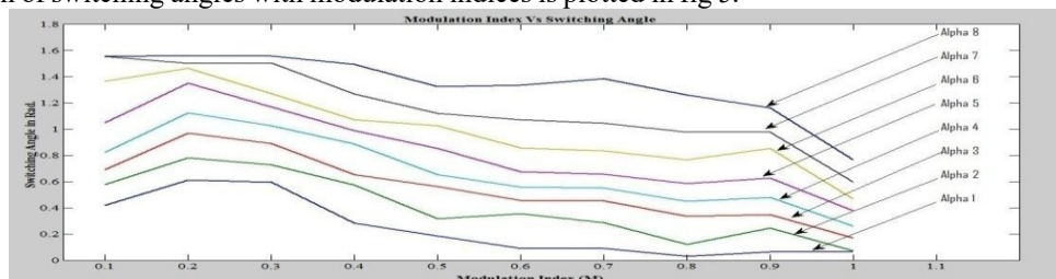
Fig. 5. Modulation Index vs. Calculated switching for seventeen level
