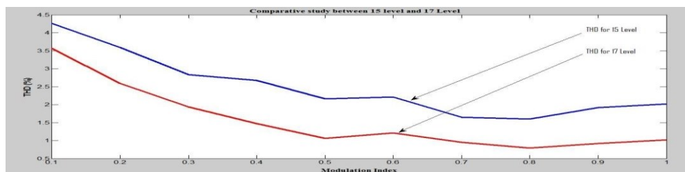
Fig. 10. Comparative study between fifteen level and seventeen level cascaded multilevel inverter
