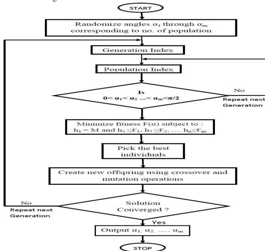
Fig.3 Flowchart of Genetic algorithm
