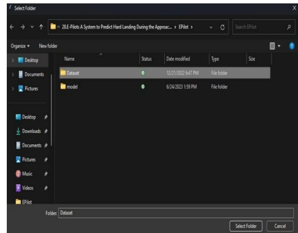
Fig.2. Loading Dataset.
