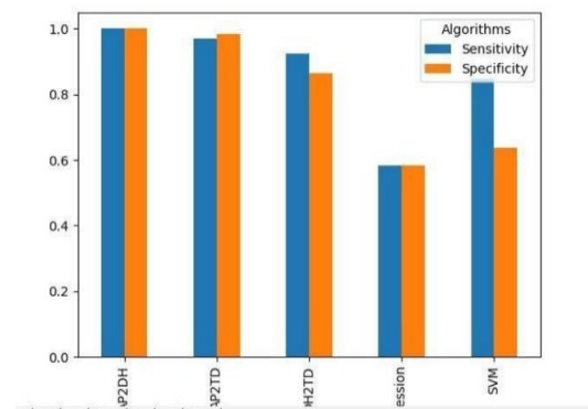
Fig.8. Output Graphs.
