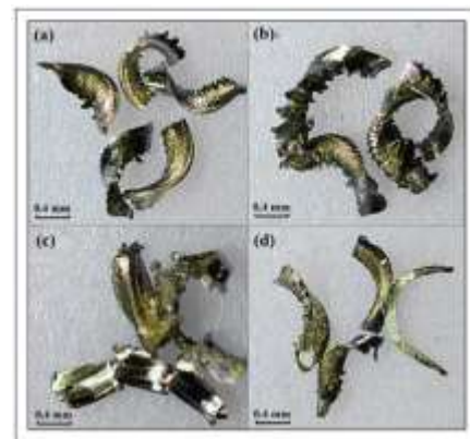
Figure 7. Chip morphology under different CL conditions:
