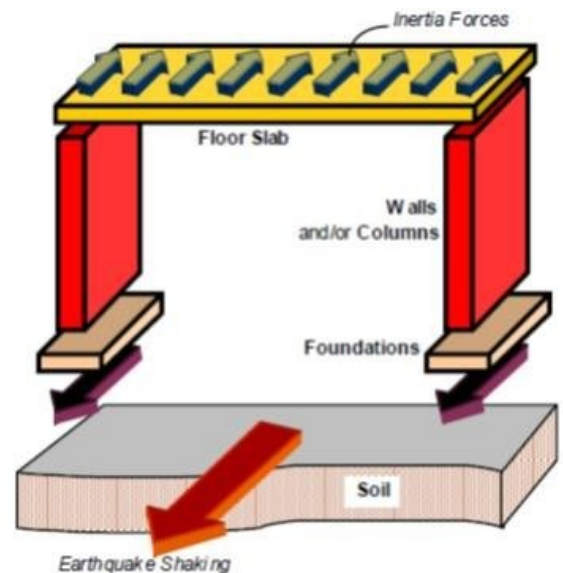
Fig.1.1. Flow of seismic inertia forces.
