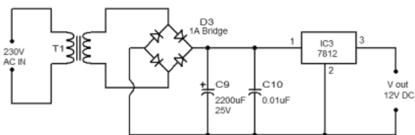
Fig 4: Circuit Diagram of Power Supply
