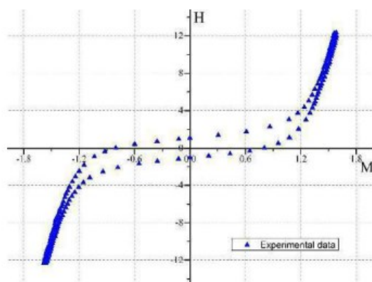
Figure 7: Reverse hysteresis of CuFe2O4 nanomagnetic compounds
