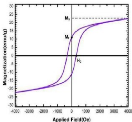
Figure 6: The hysteresis loop of CuFe2O4 nanoparticles fired at 850 0C
