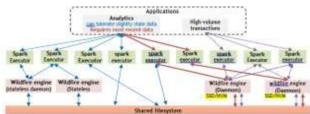
Figure 1: Wildfire Architecture.
